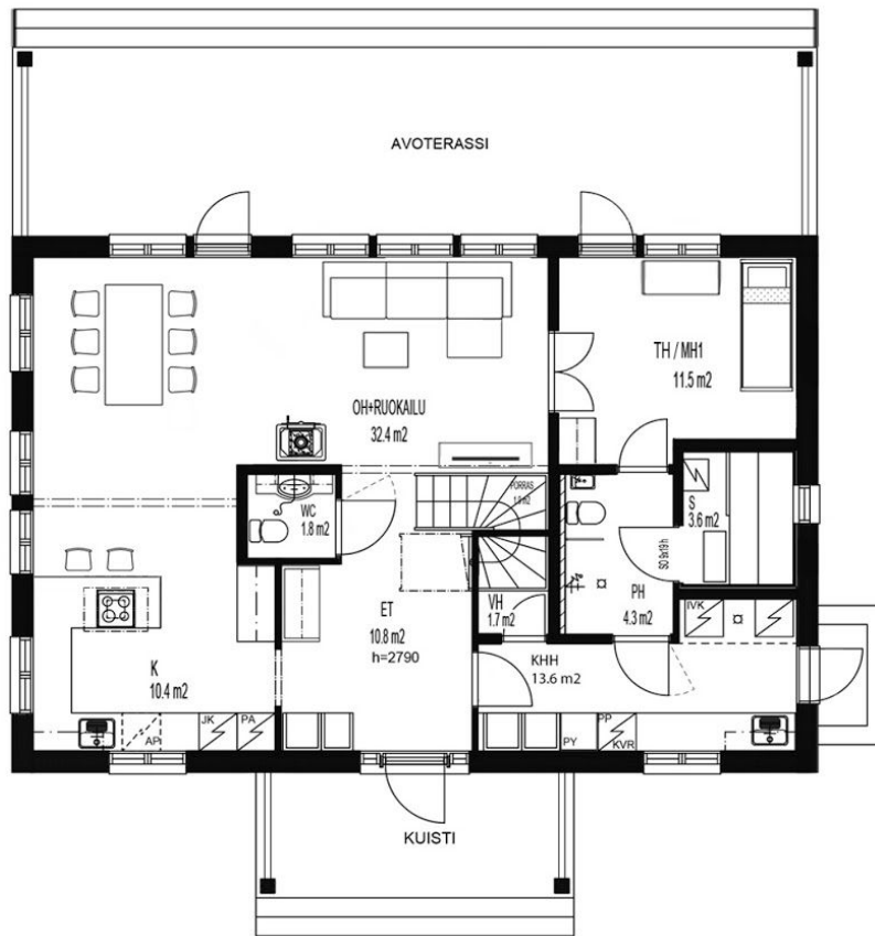
Skoone 175 Ground Floor Plan
