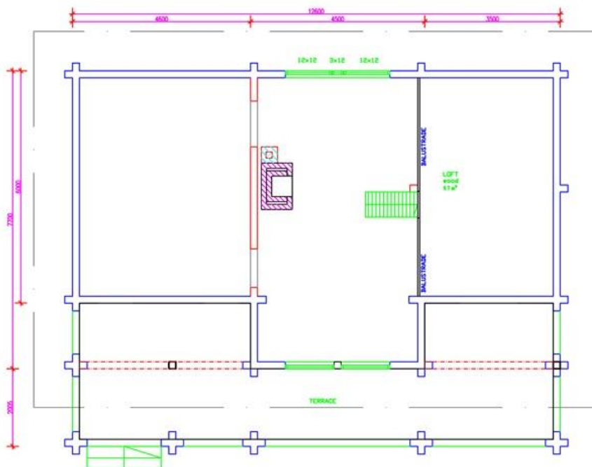
Ihana 2 First Floor Plan
