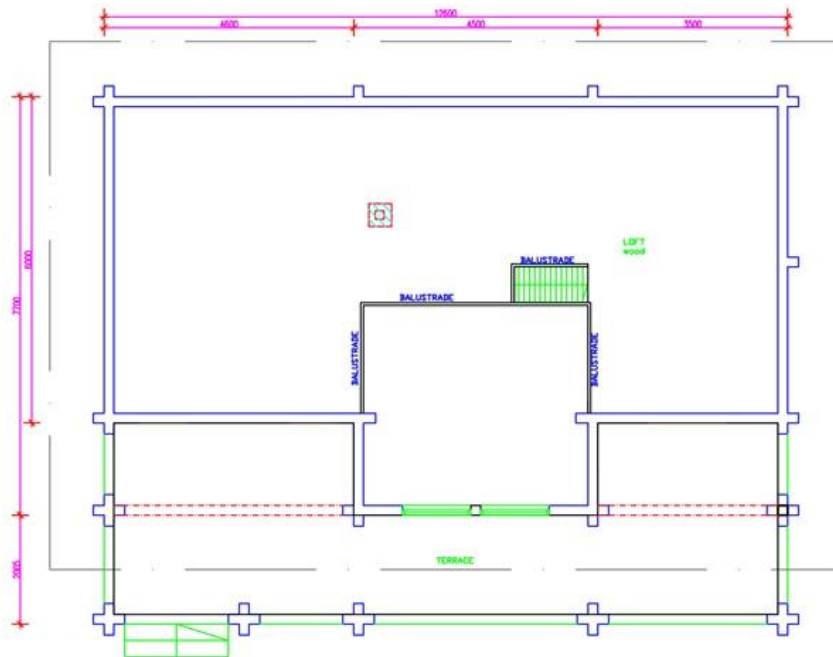
Ihana 3 First Floor Plan
