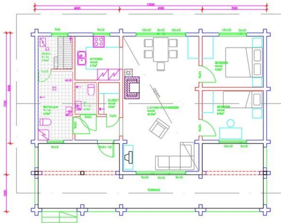
Ihana 1, 2 and 3 Ground Floor Plan (83 m2 external floor area)
