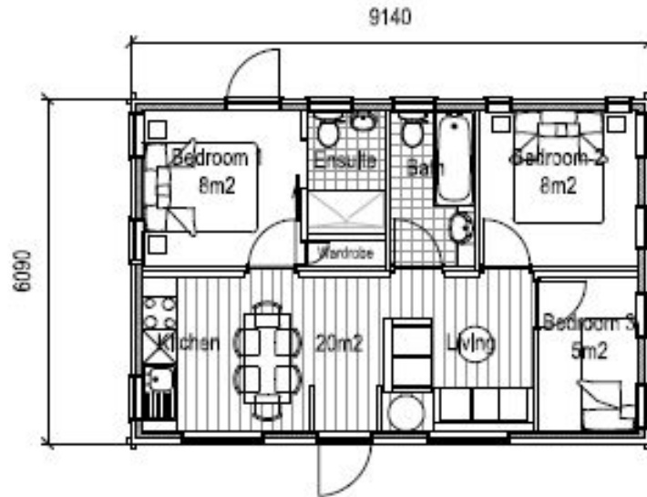
Twin unit 30 x 20 ft 3 bed internal area 50 m 2
