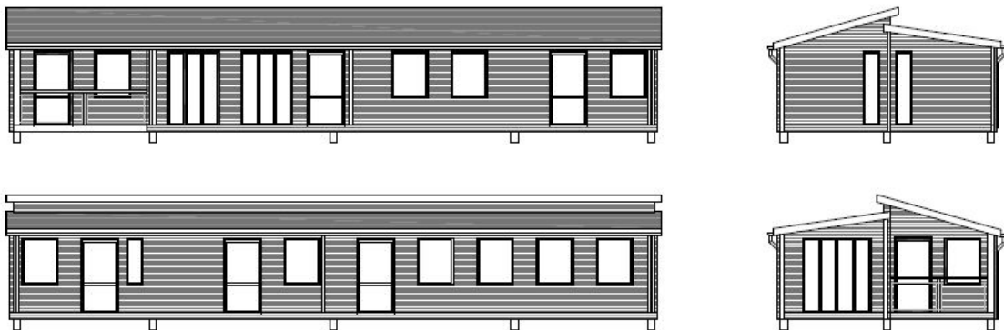
Twin Unit 60 x 20 Elevations
