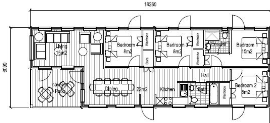
Twin Unit - 60 x 20 ft 4 bed, internal area 100m 2
